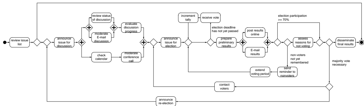
Figure 1. Example for business process control flow logic (in BPMN)
