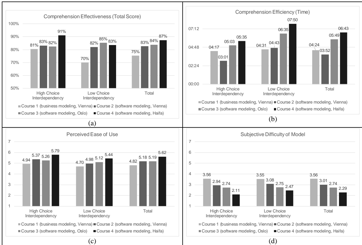
Figure 6. Results for model comprehension: (a) comprehension effectiveness (total score), (b) comprehension efficiency (time), (c) perceived ease of use, and (d) subjective difficulty of model
