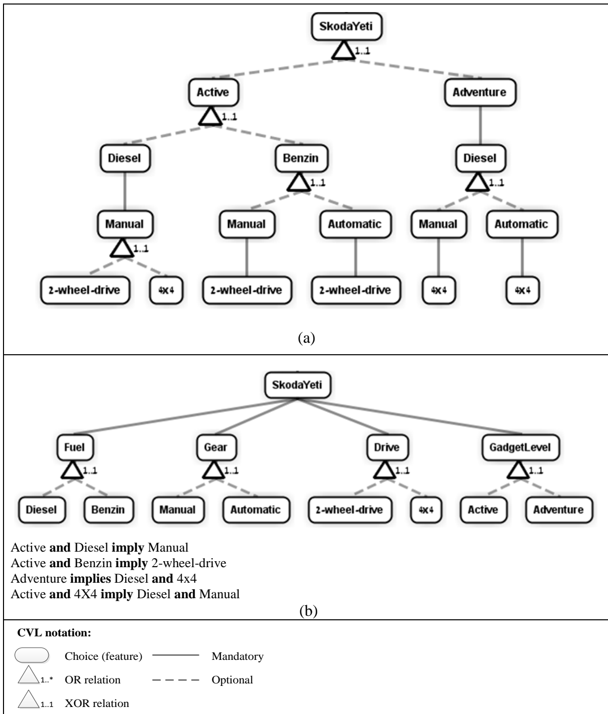
Figure 1. CVL models specifying the variability within basic choices of Skoda Yeti cars: (a) hierarchical style and (b) constrained style
