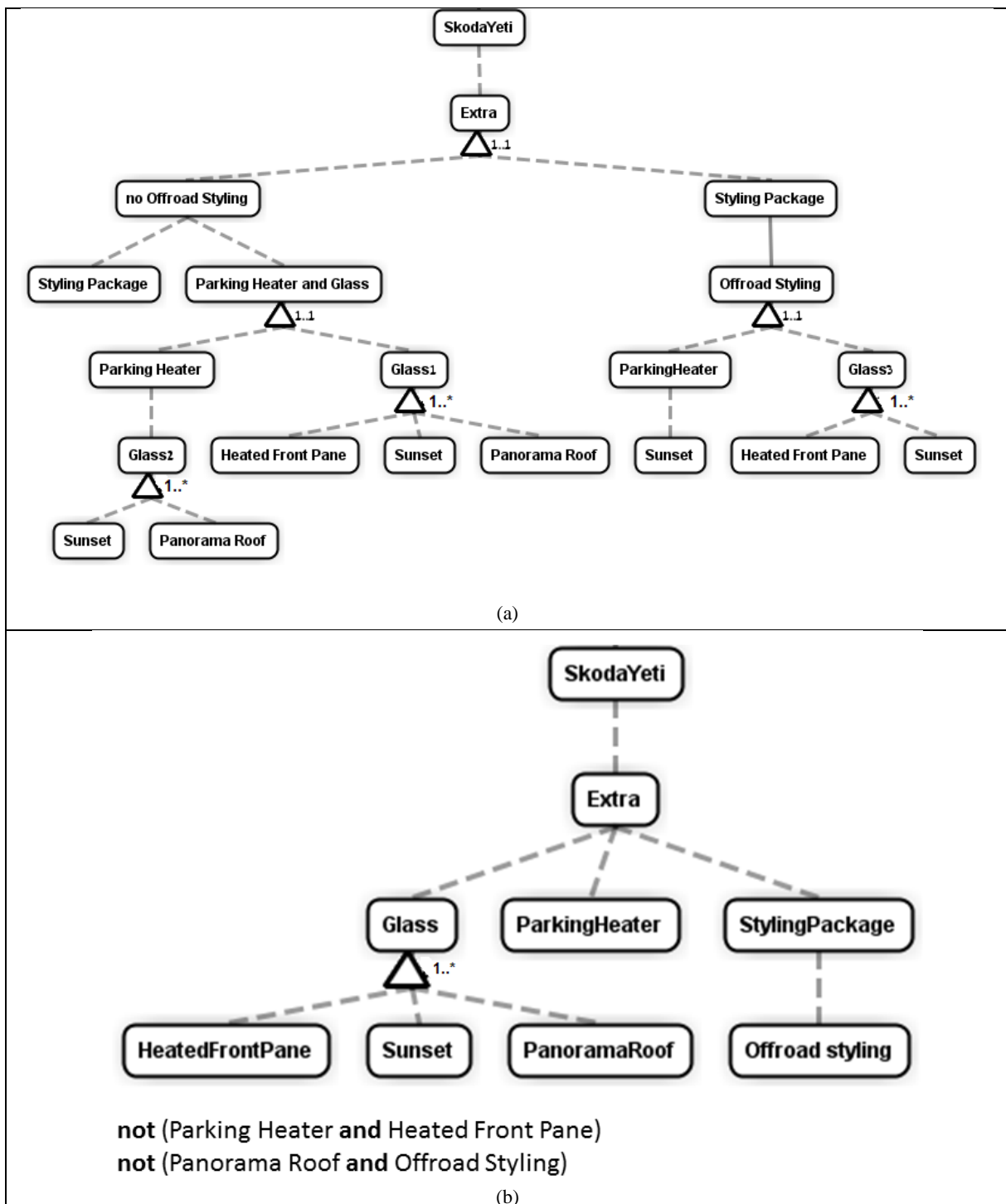
Figure 5. CVL models specifying the variability within extra choices of Skoda Yeti cars: (a) hierarchical style and (b) constrained style
