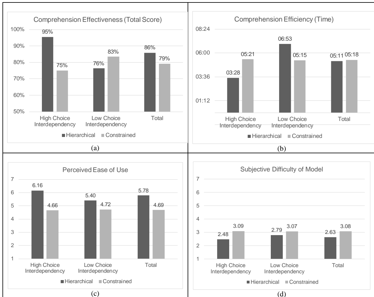
Figure 4. Results for model comprehension: (a) comprehension effectiveness (total score), (b) comprehension efficiency (time), (c) perceived ease of use, and (d) subjective difficulty of model
