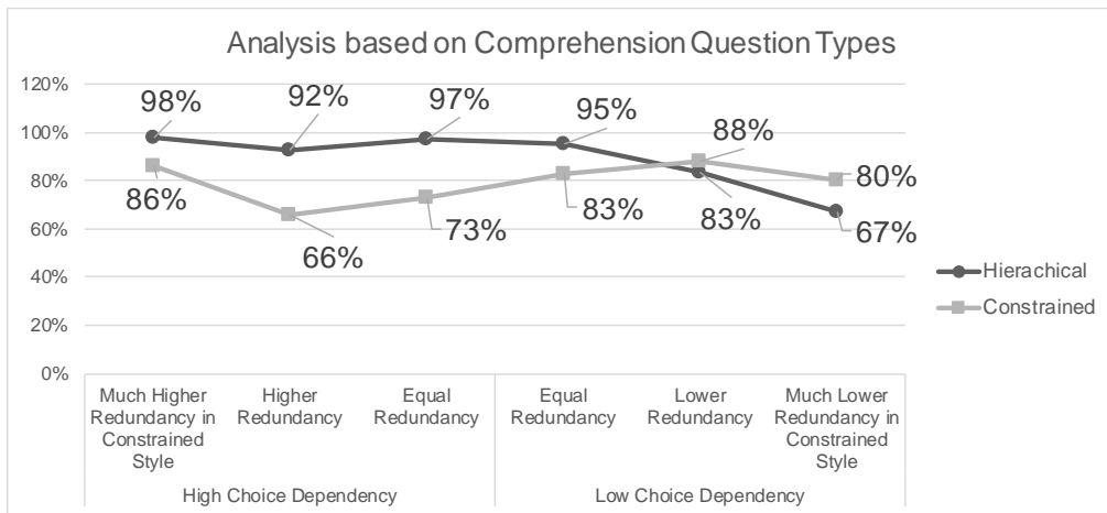
Figure 7. Redundancy in comprehension question types and comprehension effectiveness
